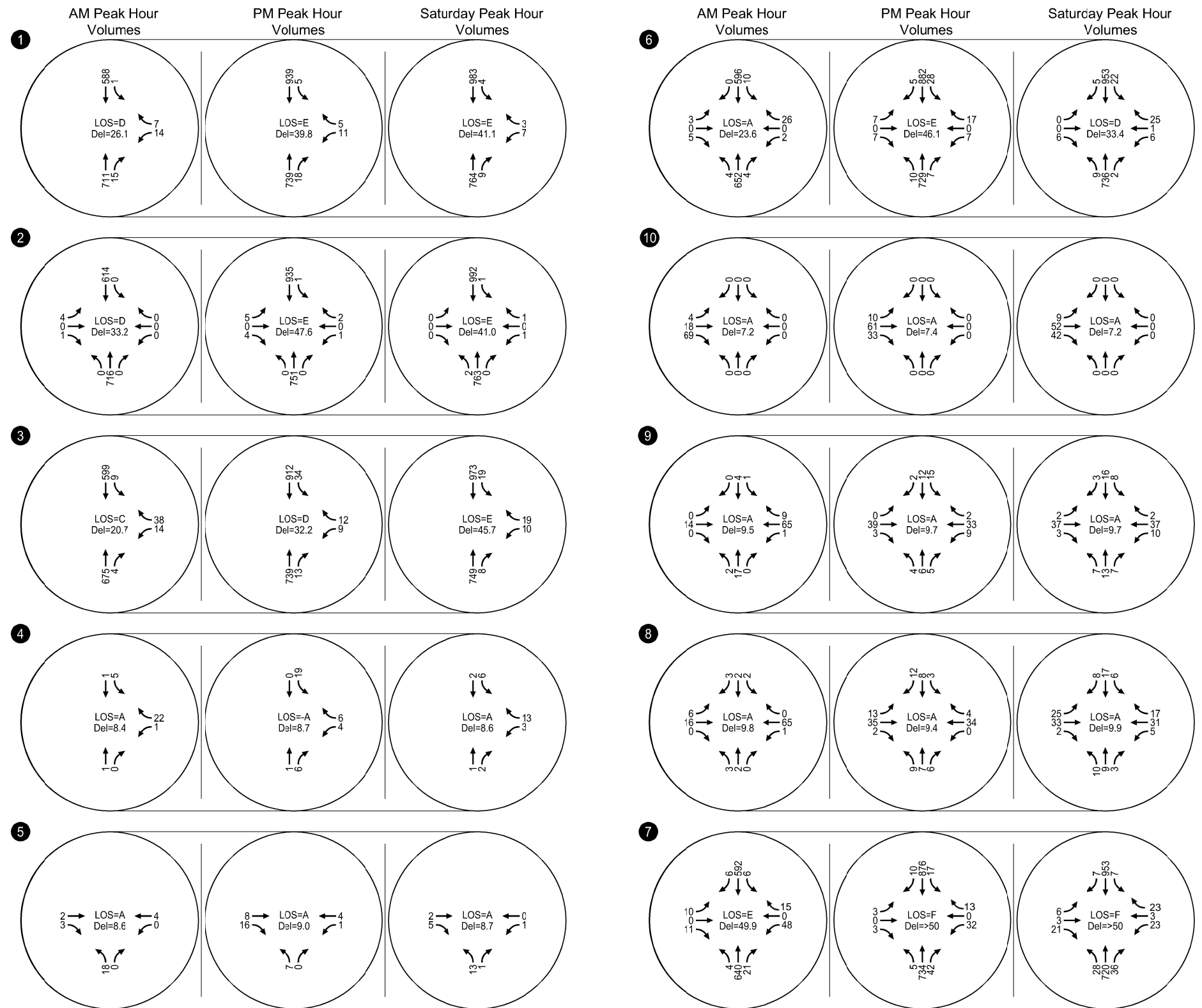
Near-Term with Project Turning Movement Volumes and Operations AM, PM, and Saturday Peak Hour Moss Beach, California
