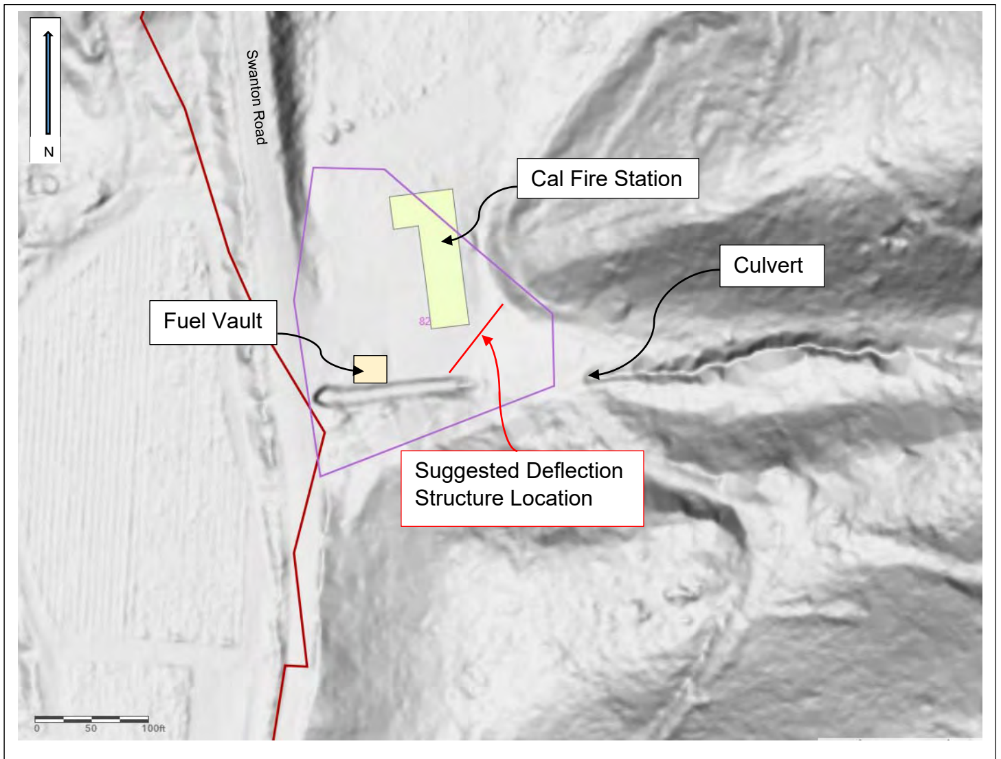
Figure 15. Site map of CAL FIRE station (VAR 82) showing the potential location of a properly designed deflection structure. The culvert denotes the location where debris could plug the structure and flow towards the station and fuel vault.
