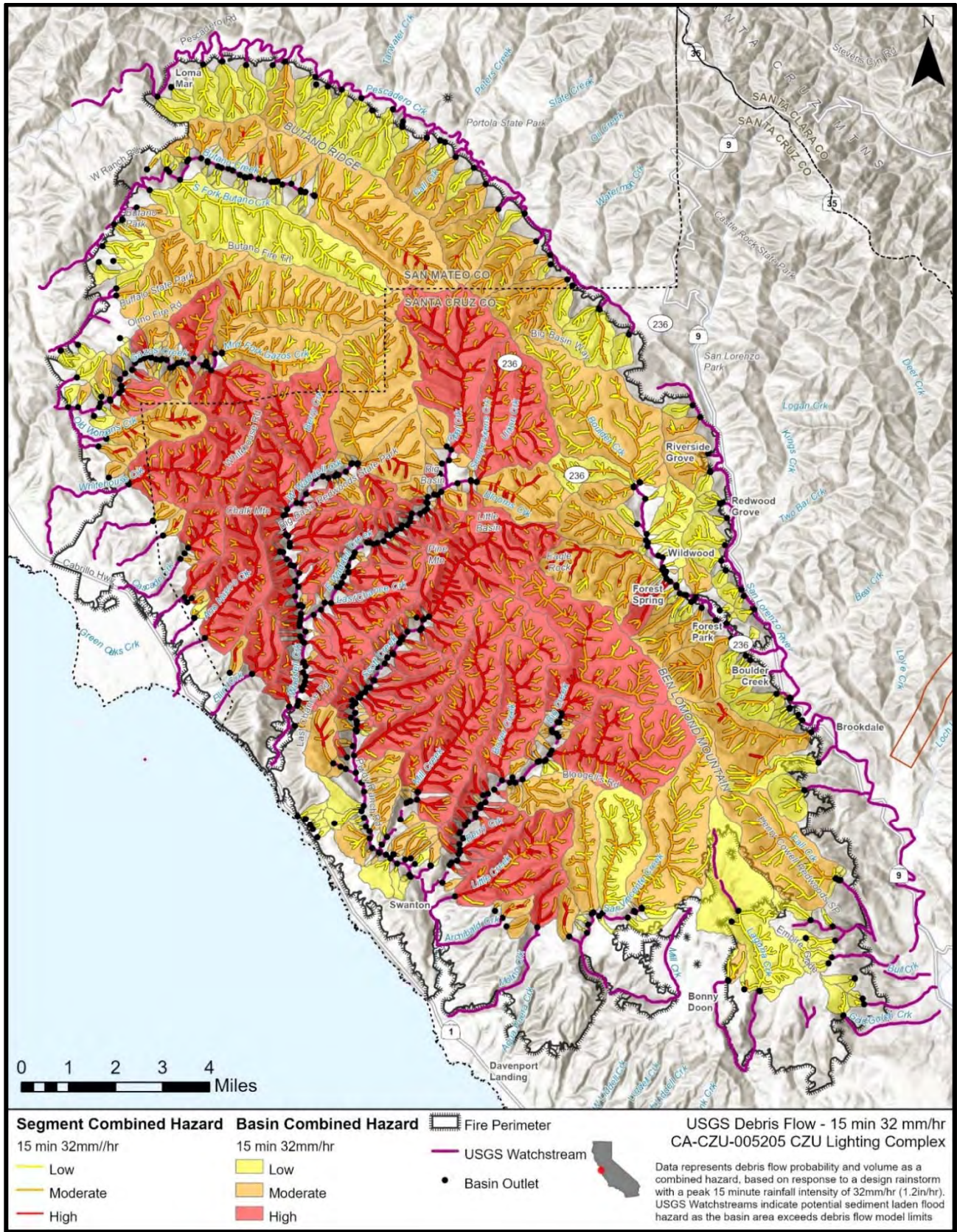
Figure 10. USGS debris flow model results for the 15-min 32 mm hr -1 , CZU Lighting Complex.
